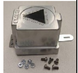
Top Kit - complete cap assembly for bare tubing
